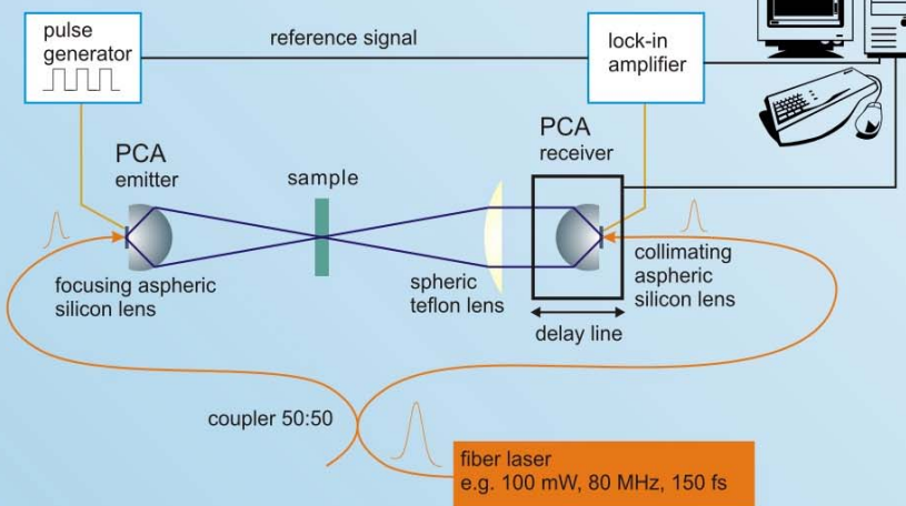
Setup with two fiber coupled antennas with a collimating and a focusing silicon lens
