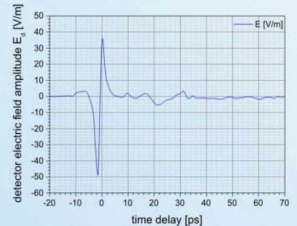
Time-domain terahertz field scan and corresponding terahertz spectrum
