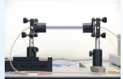
setup with two collimating silicon lenses
