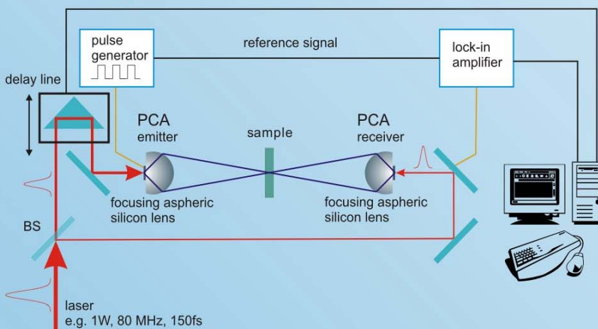
Free space setup using two antennas with focusing silicon lens
