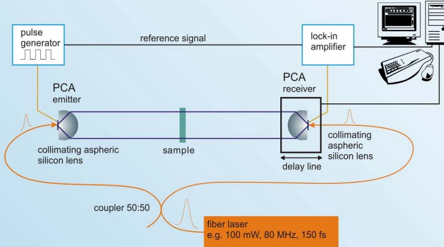
Setup with two fiber coupled antennas with collimating silicon lenses
